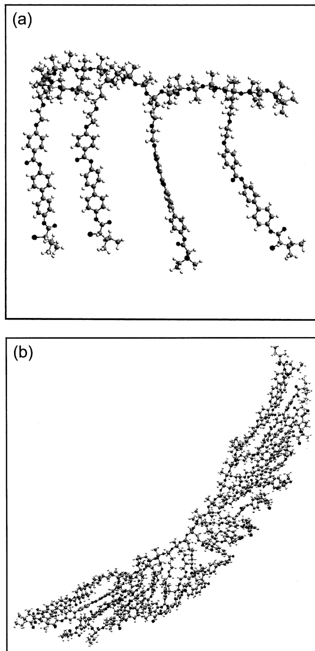
Figure 4. Lowest energy configurations of (a) PS112Bs15 and (b) PS112Bs100.
